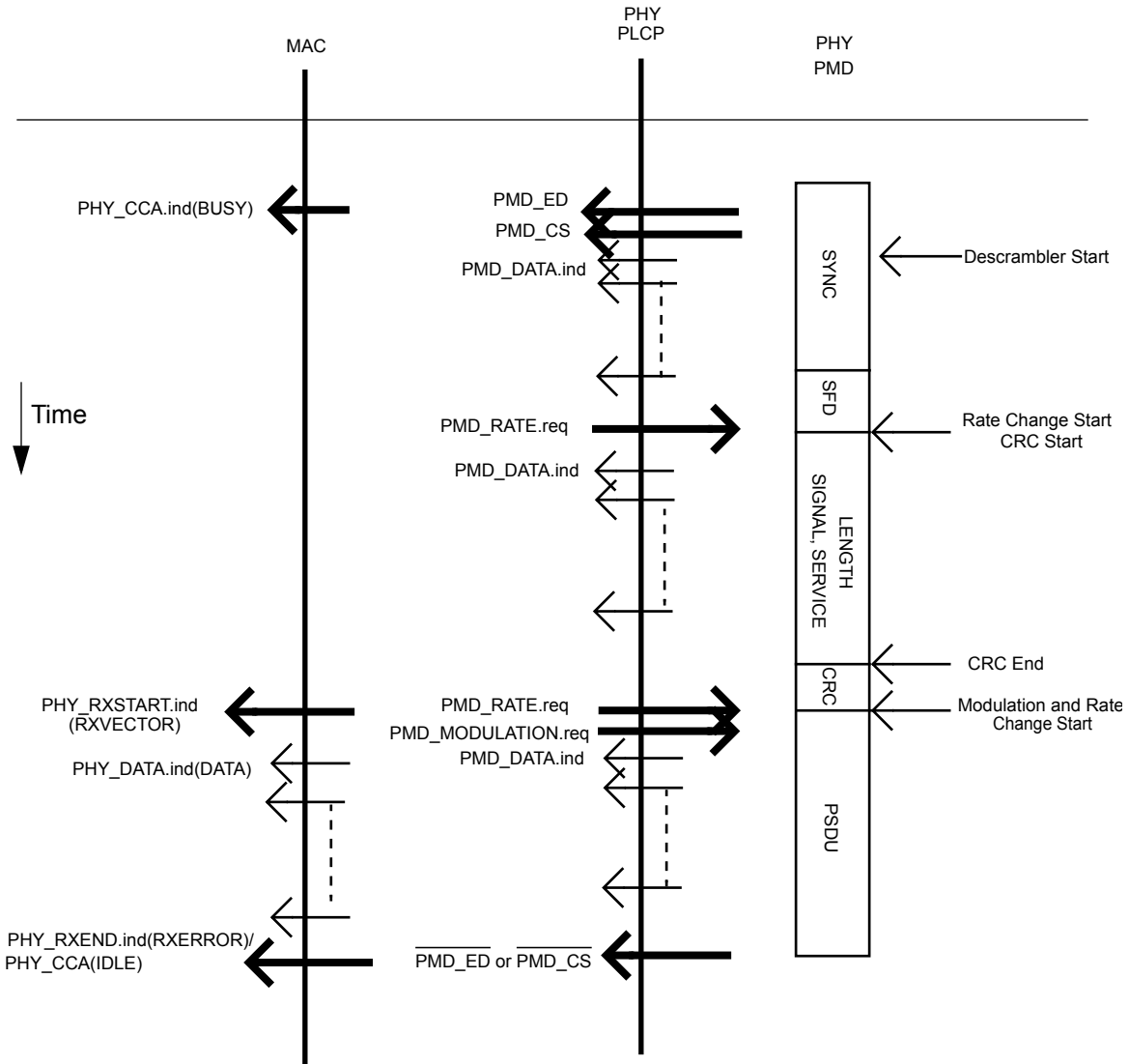
Figure 135—PLCP receive procedure
