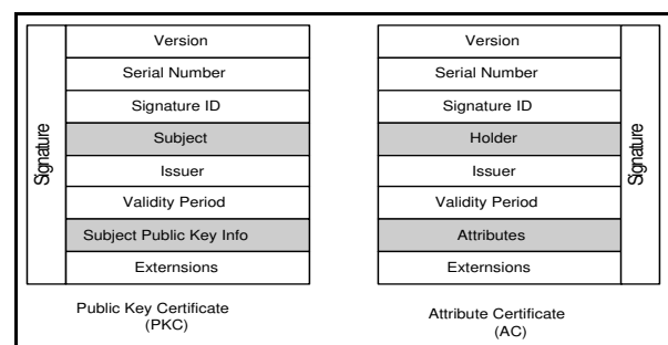
Fig. 2. PKC and Attribute certificates
