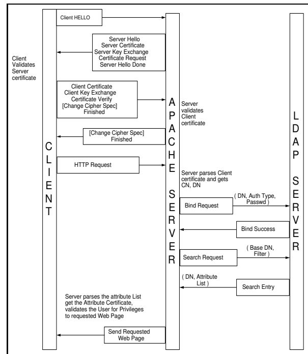
Fig. 6. Message Flow between the components
