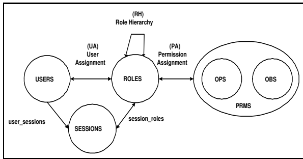
Fig. 1. Core RBAC [8]
